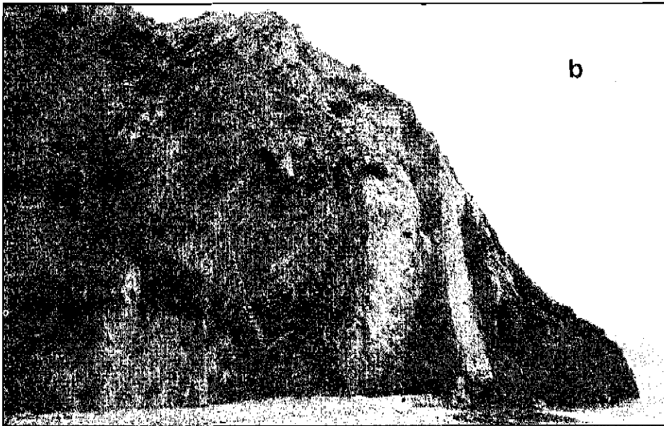
Figure 2. The sheeted nature of the pluton. a) Line drawing of photograph originally published by Shepard & co-authors (1939) showing dikes exposed along a 25 km segment of the Palisades near the southeastern end of the island, b) Steeply northwest-dipping dikes at mouth of Silver Canyon. Person in middle-ground for scale. Photographer is facing east
