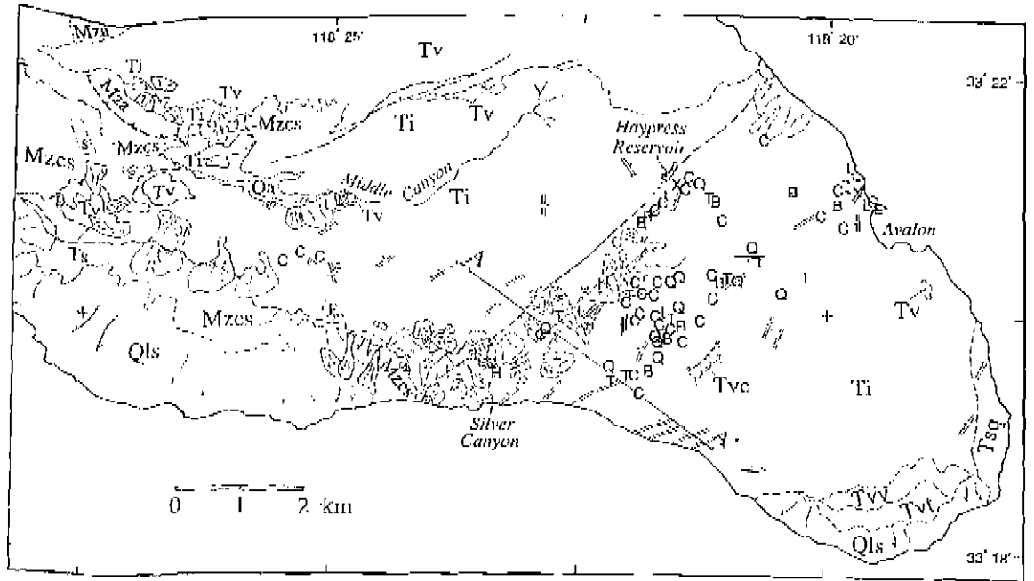
Figure 3. Generalized bedrock geology of the pluton and surrounding units, southeastern Santa Catalina Island. Light lines represent dispositional or intrusive contacts, heavy lines represent faults, solid where exposed, dashed where approximately located, dotted where covered. Teeth on upper plate of thrust fault. Short parallel lines represent trends of steeply dipping dikes, or outcrops of dikes in Palisades; small ticks on the dike symbols represent the direction of dip. Rock units: Ts , Tertiary tuffaceous siltstone and calcarenite; Tvc , Tertiary volcanoclastic siltstones to conglomerates less than 19 Ma; Tv , Tertiary volcanic rocks 19-12 Ma, undifferentiated, mostly porphyritic and sometimes vesicular; Tvf , Tertiary andesitic flow rocks, frequently with asymmetric vesicles or amygdules; Tvt , Tertiary crystal-lithic-vitric andesitic tuff; Ti , Tertiary intrusive rocks—hypabyssal (biotite-)(augite-) hornblende quartz diorite porphyry; Tsq , Tertiary East End Quarry sequence, including San Onofre Breccia and underlying strata; Mzcs , Mesozoic or older Catalina Schist—greenschist and blueschist lithologies; Mza , Catalina Schist—garnet-hornblende amphibolite; s , serpentinite. Xenoliths: B , graphitic albite-biotite greyschist; C , albite-chlorite greenstone; H , garnet-hornblende amphibolite; L , lawsonite-talc-glaucophane blueschist; Q , vein quartz; T , actinolite-talc greenschist; X , San Onofre Breccia. For a description of rock types in the Catalina Schist, refer to Platt (1976). A-A': line of schematic cross section shown in Figure 4. Geology significantly modified from Smith (1897), Bailey (1941) and Vedder & co-authors (1979). The new mapping is by S.Q. Boundy-Sanders (1986-87), J. G. Vedder (1986-87), C. O. Sanders (1986) and R.G. Bohannon (1987).
