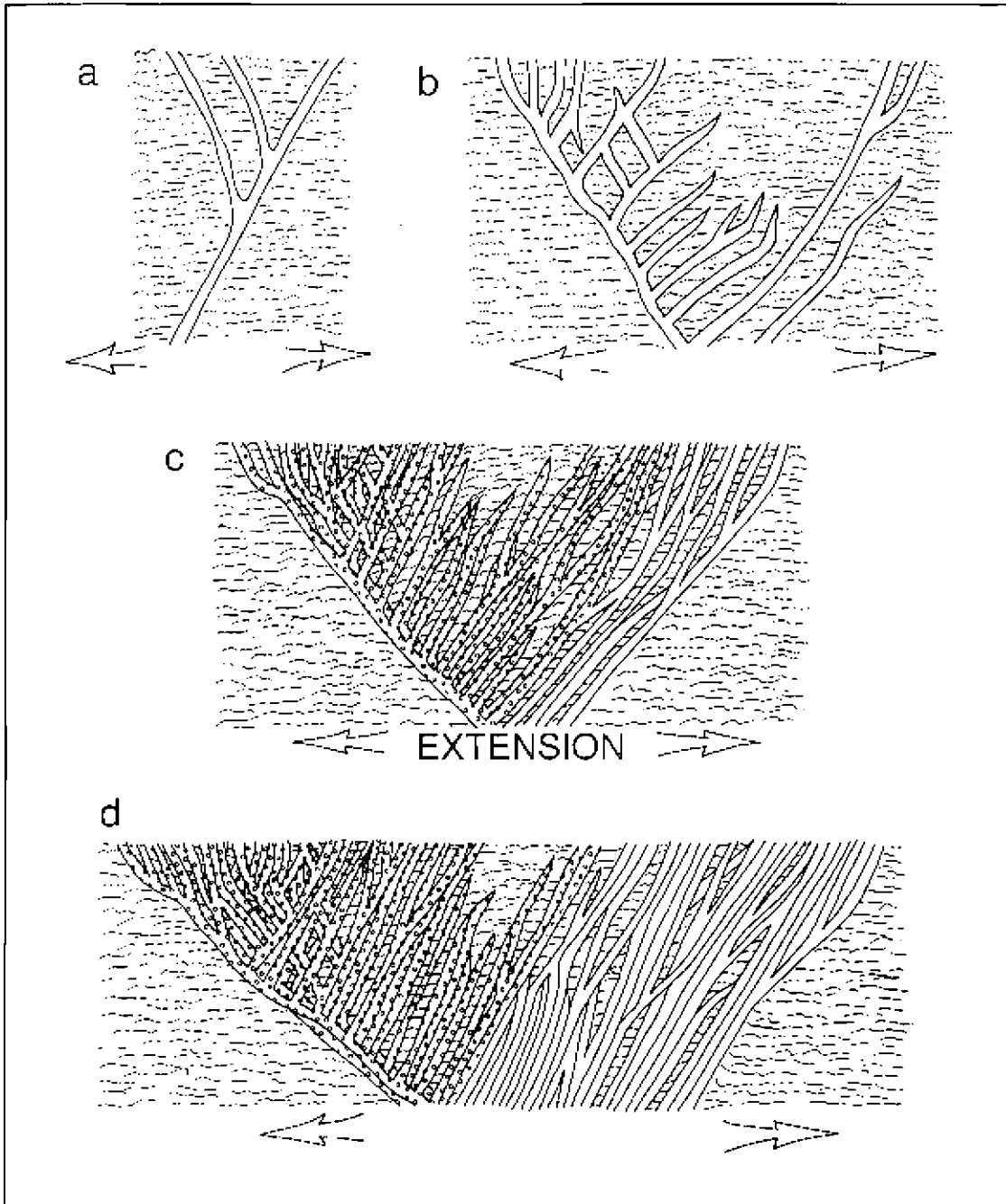
Figure 6. Idealized models of extension that produces a swarm of dikes, such that different dikes have varying attitudes from the time of intrusion. Symbols are the same as those used in Figure 5. a) Structure of the Comstock Lode, Nevada (Becker 1882); b) clay-cake experiment (Cloos 1971) to explain the pattern of faults around the Gulf of Mexico; c) and d) hypothetical result of continued spreading of the clay cake and filling of fractures as they are produced. Result is a dike swarm produced by extension and intrusion, limited assimilation, and upward transport and ejection of xenoliths. Xenoliths are most abundant in the zone where dips reverse. This zone represents the area of initial extension where the greatest number of xenoliths and screens were created. Vertical measurement of each panel is approximately 2-4 km.
