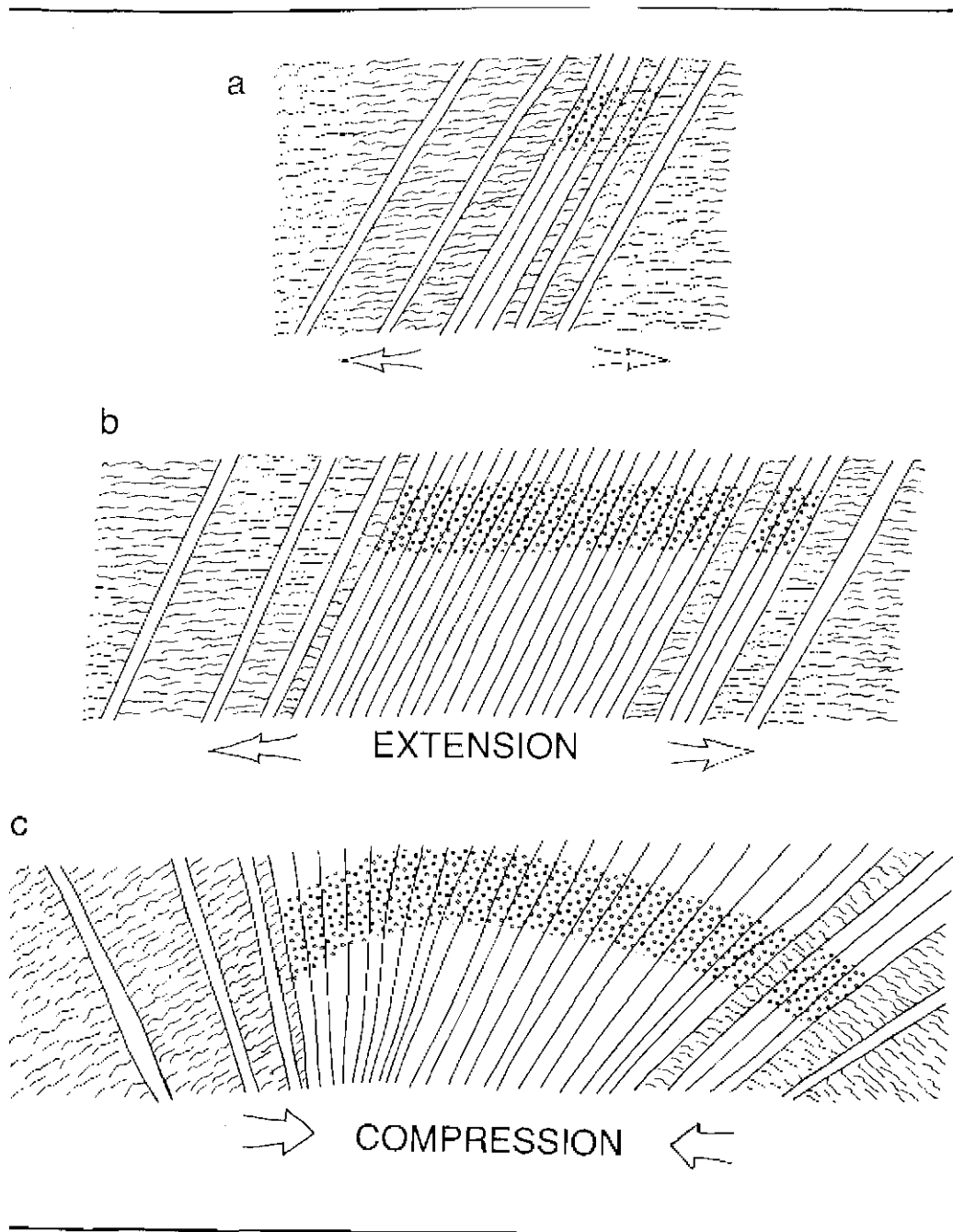
Figure 5. One model of extension that might produce a swarm of sheeted dikes. Open circles indicate zone that contains xenoliths; wavy lines, country rock; and parallel lines, dikes, a) Fractures nucleate in a single orientation, which is maintained by b) subsequent episodes of fracturing and intrusion, c) Later antiformal folding produces the change in attitudes of dikes over space. Xenoliths concentrate by isostasy at a particular level in the dikes. Vertical measurement of each panel is approximately 2-4 km. Foliation in the Catalina Schist is for illustrative purposes only; the schist in reality has a much more complex structure.
